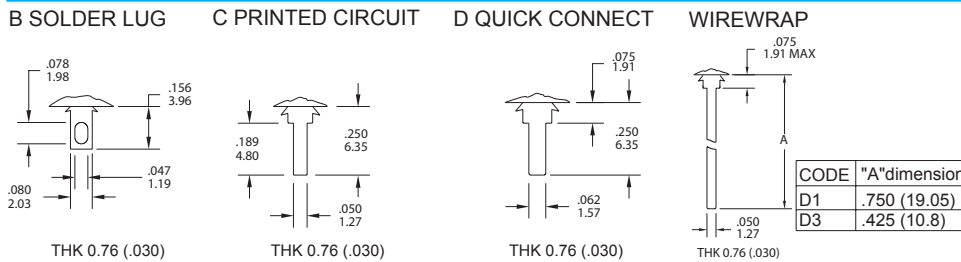
without lock ring
